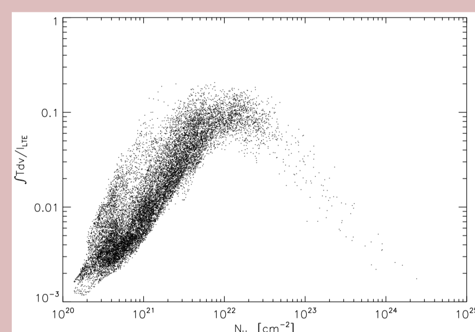
Integrated line intensity of the 13 CO 3-2 line relative to the LTE intensity for the same model.
