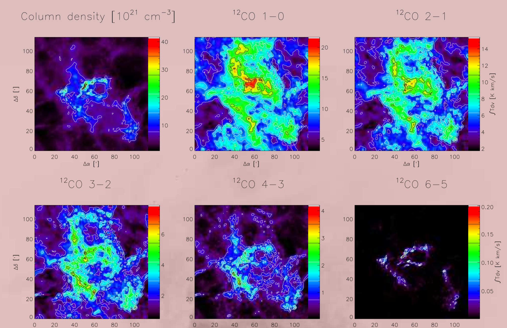
12 CO maps in the equivalent transitions computed for the same turbulence model
