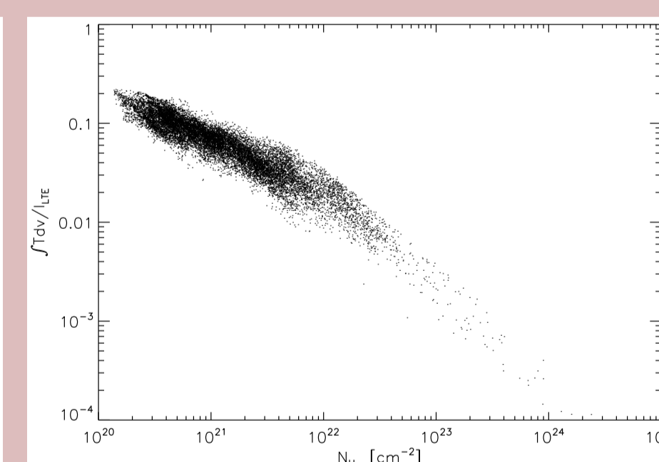
Integrated line intensity of the 12 CO 1-0 line relative to the LTE intensity for the same model.
