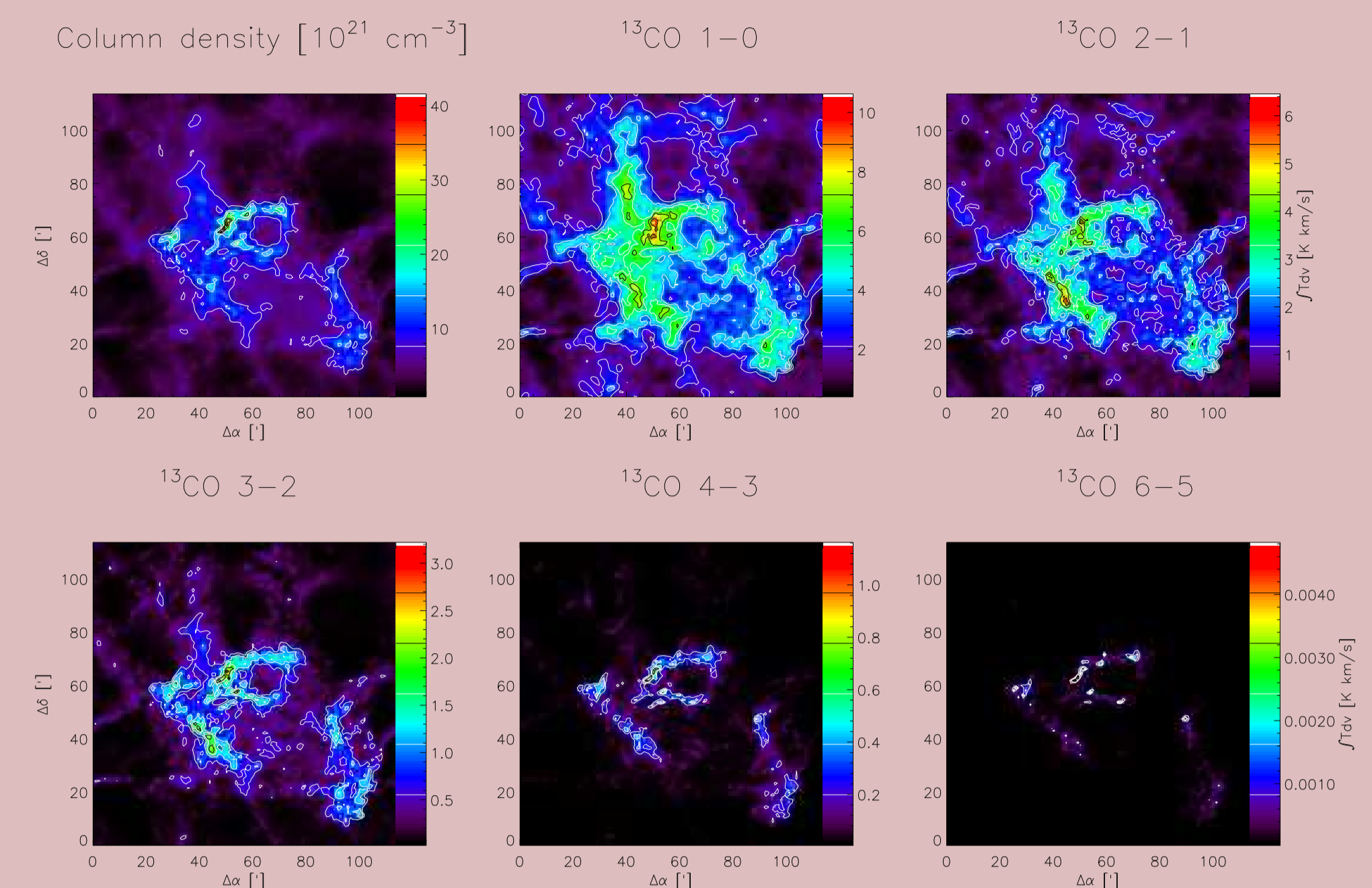
Column density and 13 CO maps in different transitions for a large-scale driven hydrodynamic turbulence model
