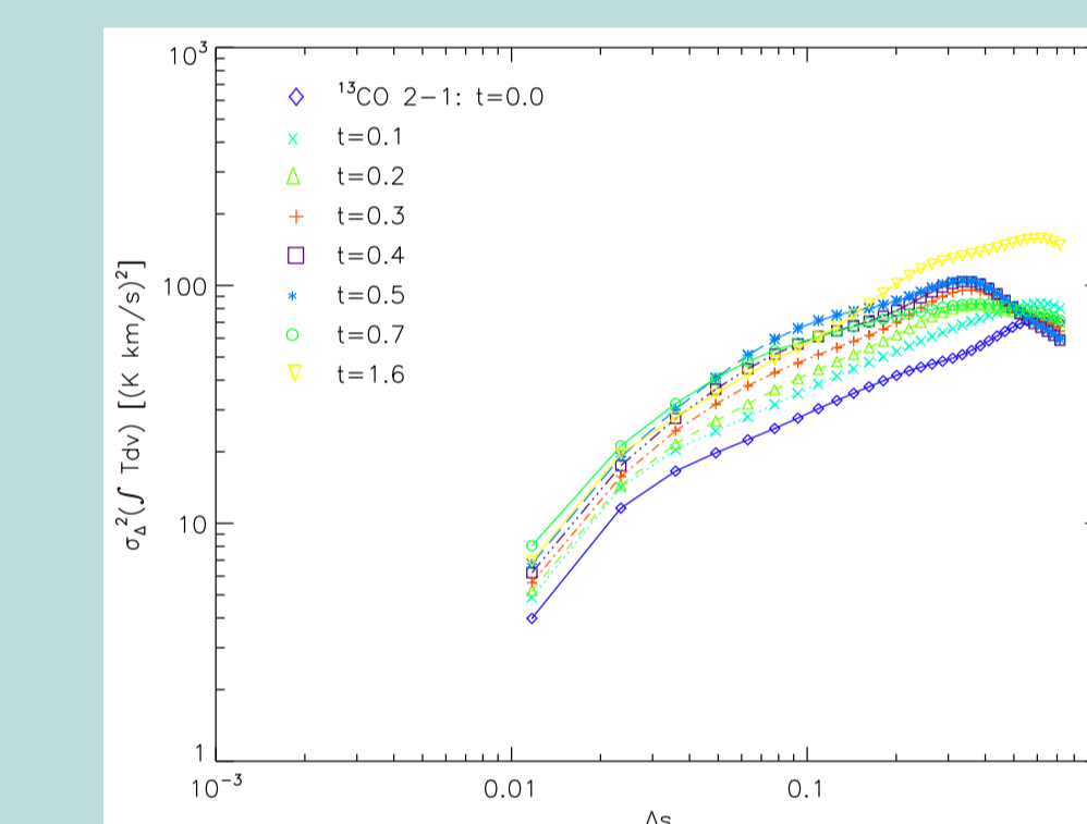
Evolution of the Δ-variance spectra of the corresponding 13 CO 2-1 maps during the collapse
