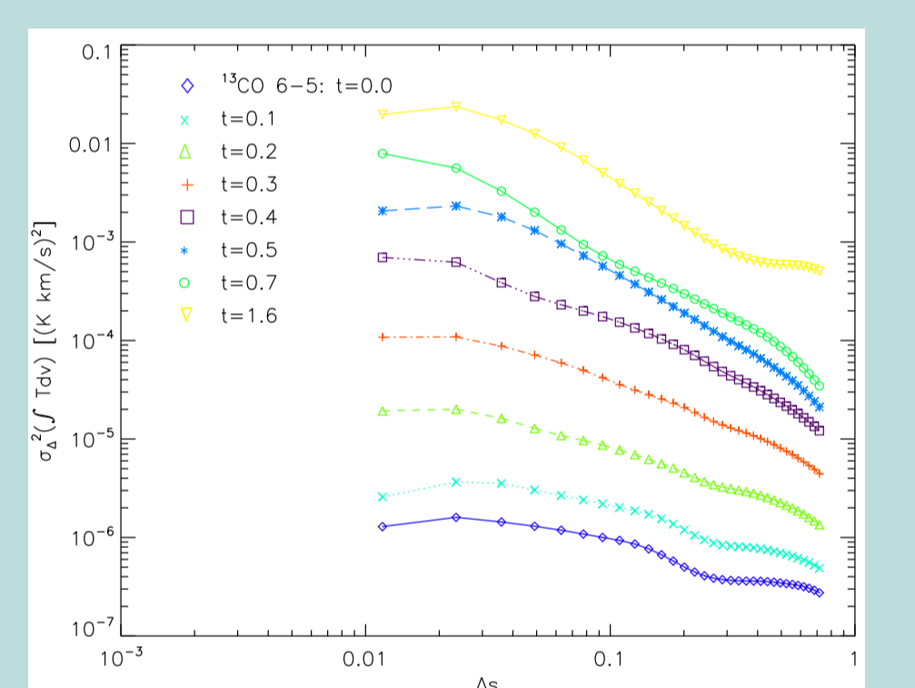
Evolution of the Δ-variance spectra of the corresponding 13 CO 6-5 maps
