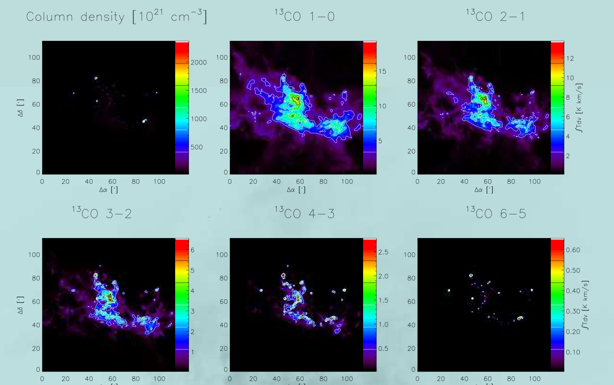
Column density map and 13 CO maps in different transitions for the turbulence model shown on the left after one free-falling time of gravitational collapse.
